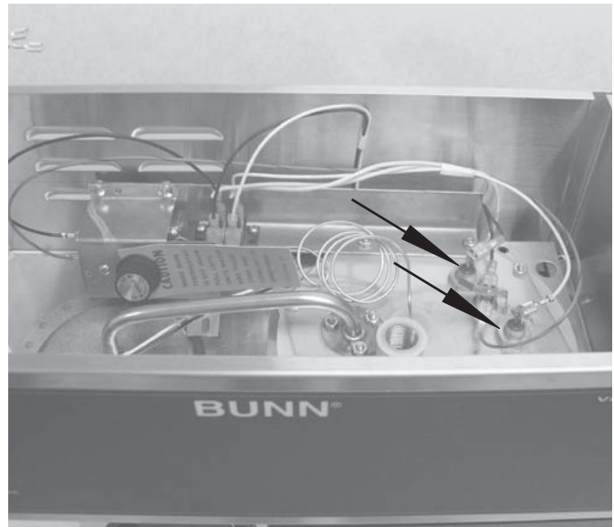
FIG. 7 TANK HEATER
